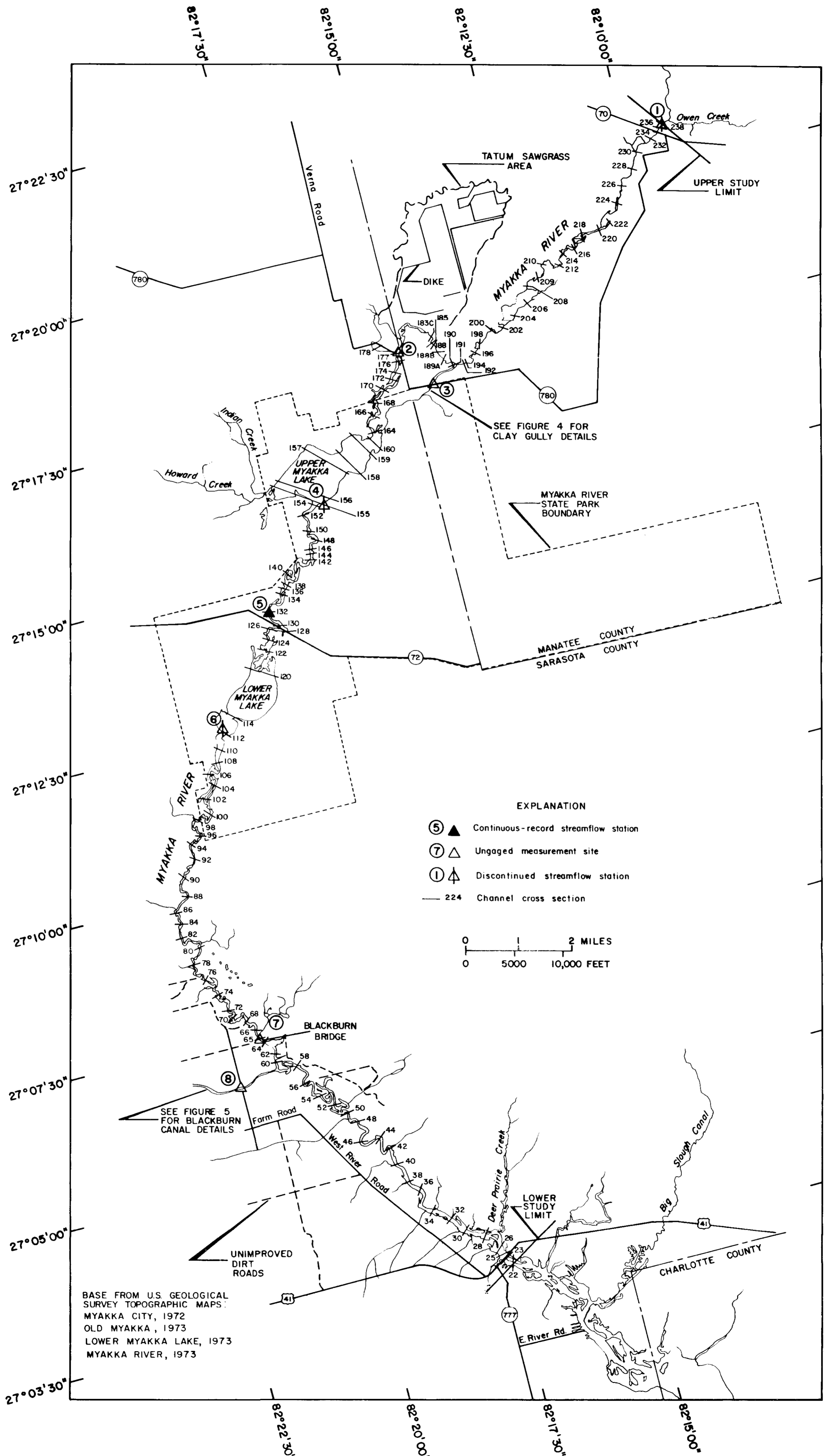
Figure 2. --Myakka River study reach showing approximate cross-section locations
